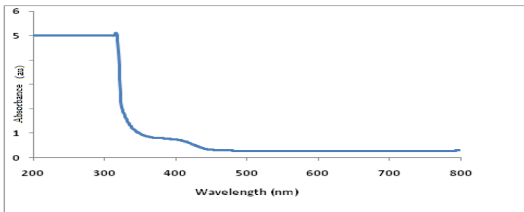
Figure B3.UV Visible absorbance Spectra of Zinc doped CdS thin films prepared at pH 12 (60 minutes)
