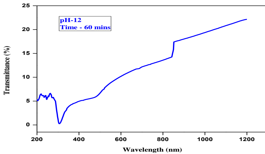
Figure B2.Transmittance Spectrum of CdS thin films prepared at pH 12 (60 minutes)
