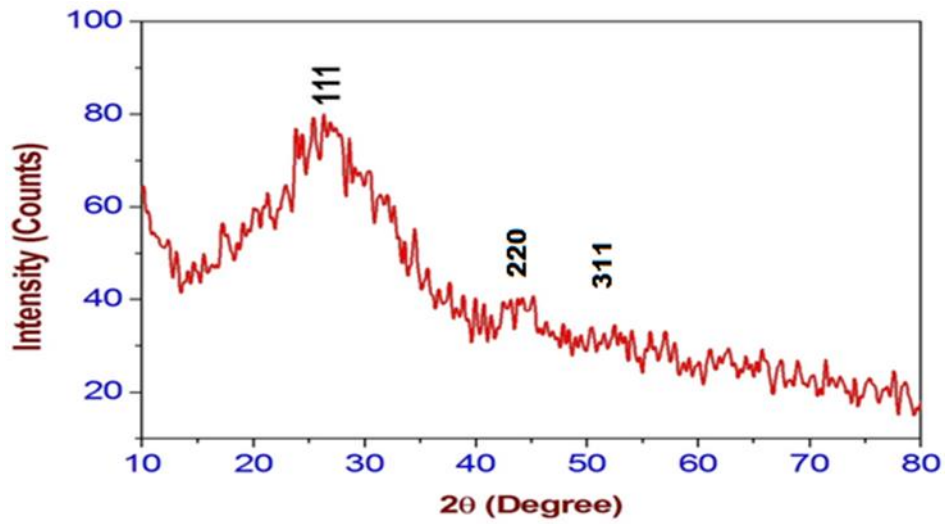
Figure B1.X-ray Diffraction spectra of Zinc doped CdS thin films prepared at pH 12 (60 minutes)
